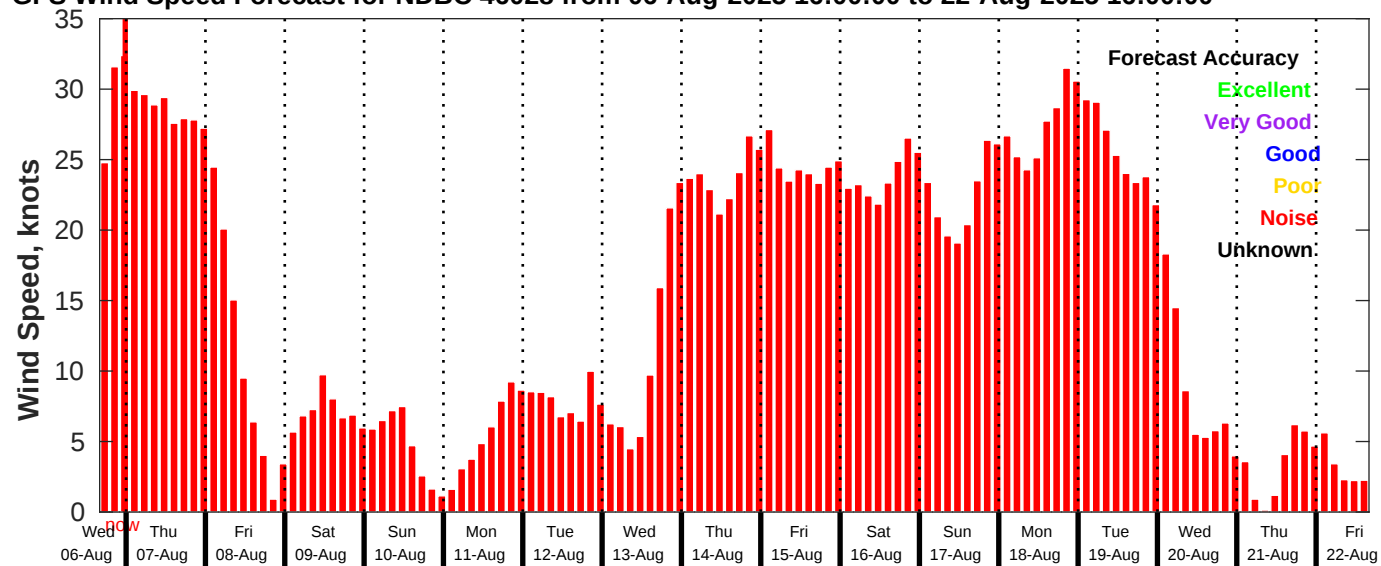
GFS Wind Speed Forecast for NDBC 46028 from 06-Aug-2025 16:00:00 to 22-Aug-2025 16:00:00
