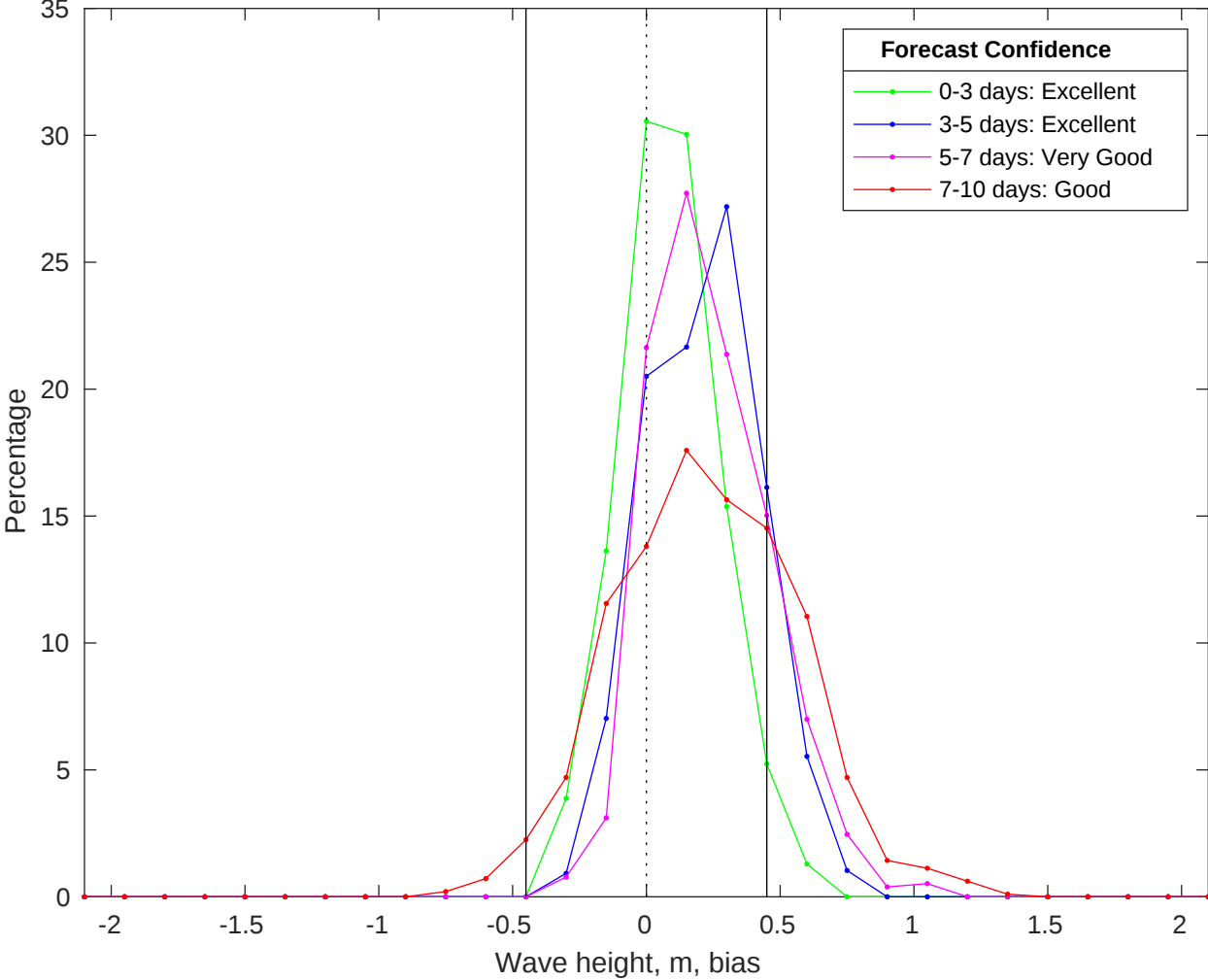
NDBC 46054 vs CMEMS Waves Bias Histogram: 07-Aug-2025
