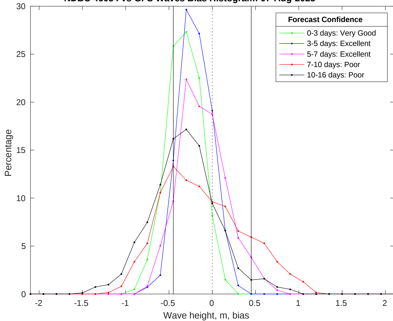
NDBC 46054 vs GFS Waves Bias Histogram: 07-Aug-2025
