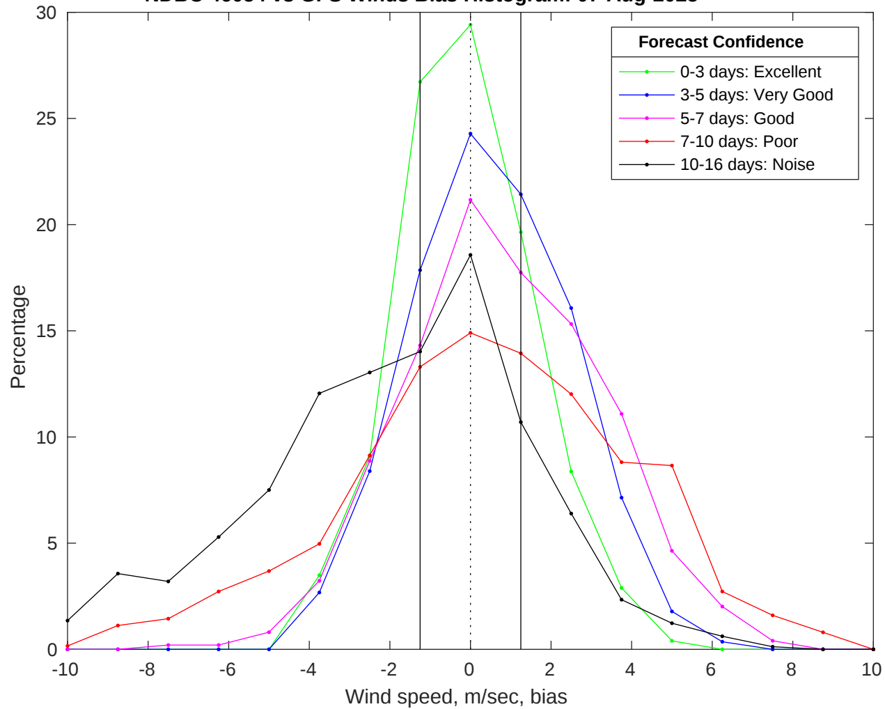
NDBC 46054 vs GFS Winds Bias Histogram: 07-Aug-2025
