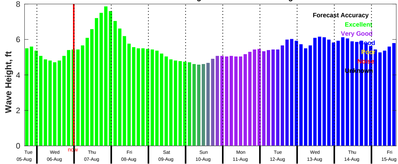
CMEMS Wave Forecast for NDBC 46054 from 05-Aug-2025 16:00:00 to 15-Aug-2025 16:00:00
