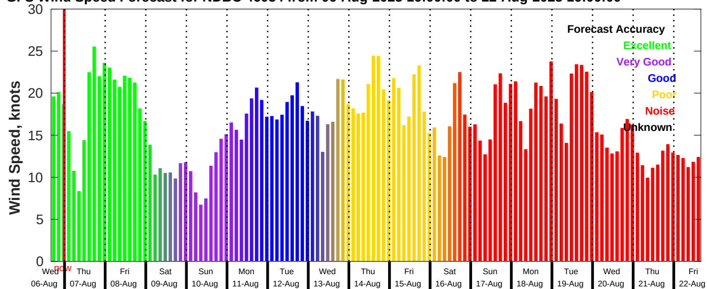
GFS Wind Speed Forecast for NDBC 46054 from 06-Aug-2025 16:00:00 to 22-Aug-2025 16:00:00
