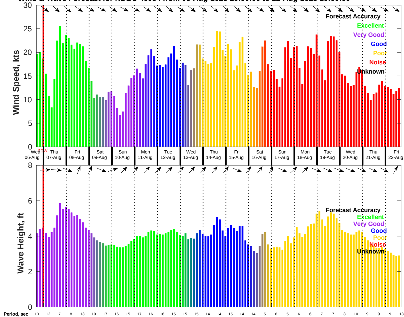
Wind & Wave Forecast for NDBC 46054 from 06-Aug-2025 16:00:00 to 22-Aug-2025 16:00:00
