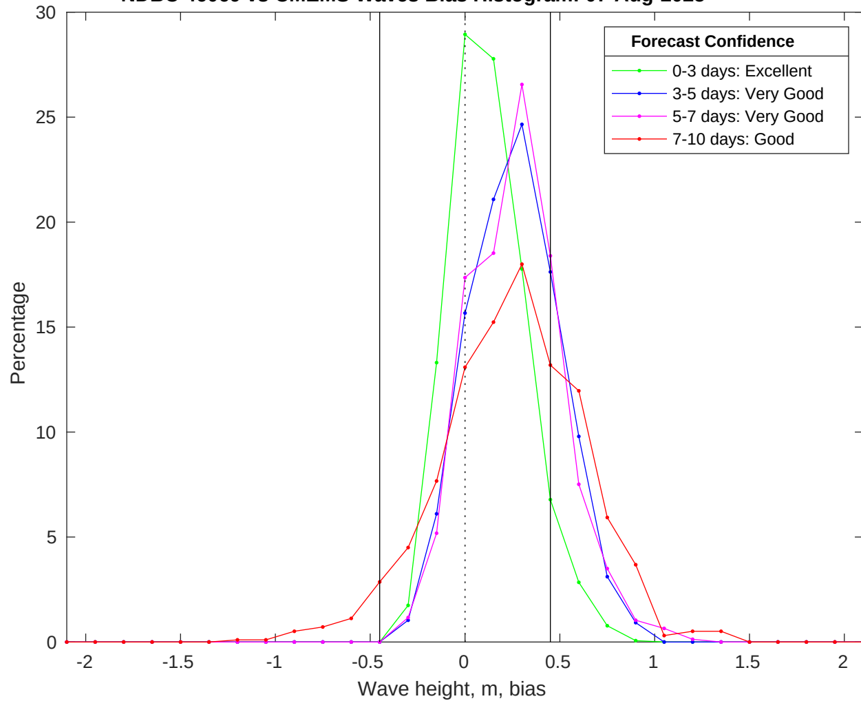
NDBC 46069 vs CMEMS Waves Bias Histogram: 07-Aug-2025
