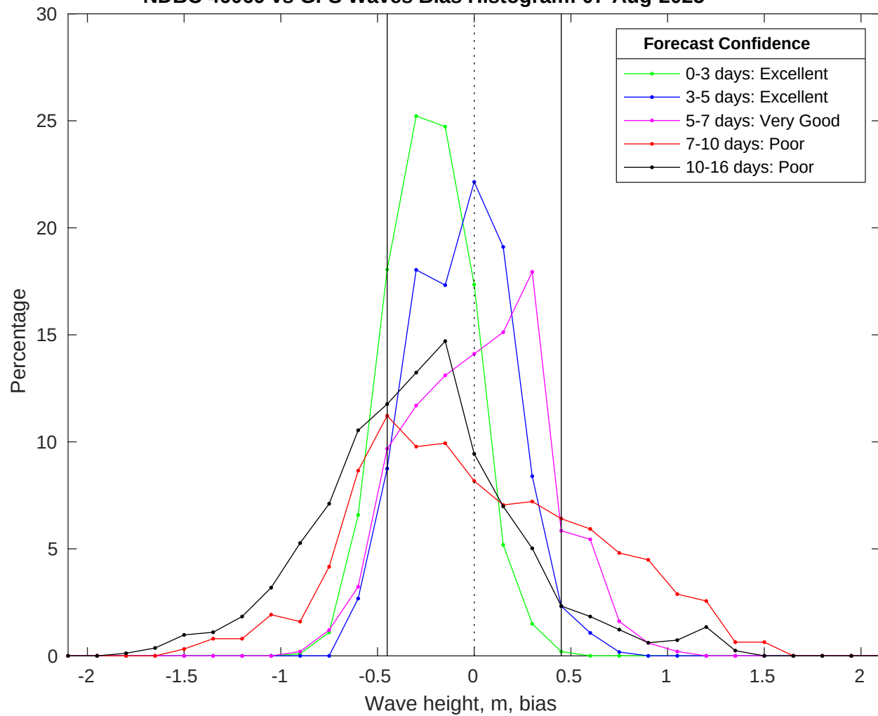
NDBC 46069 vs GFS Waves Bias Histogram: 07-Aug-2025
