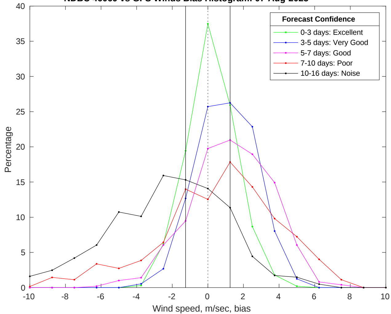
NDBC 46069 vs GFS Winds Bias Histogram: 07-Aug-2025
