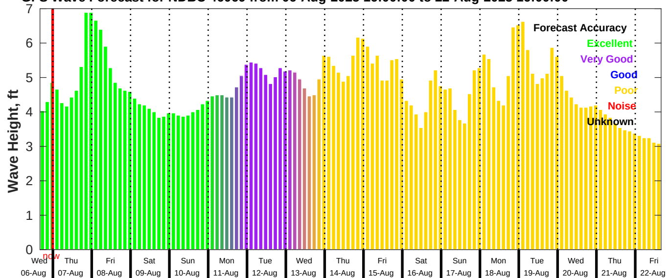
GFS Wave Forecast for NDBC 46069 from 06-Aug-2025 16:00:00 to 22-Aug-2025 16:00:00
