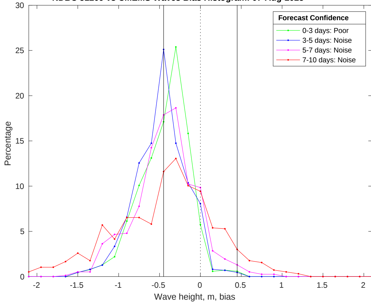
NDBC 51209 vs CMEMS Waves Bias Histogram: 07-Aug-2025
