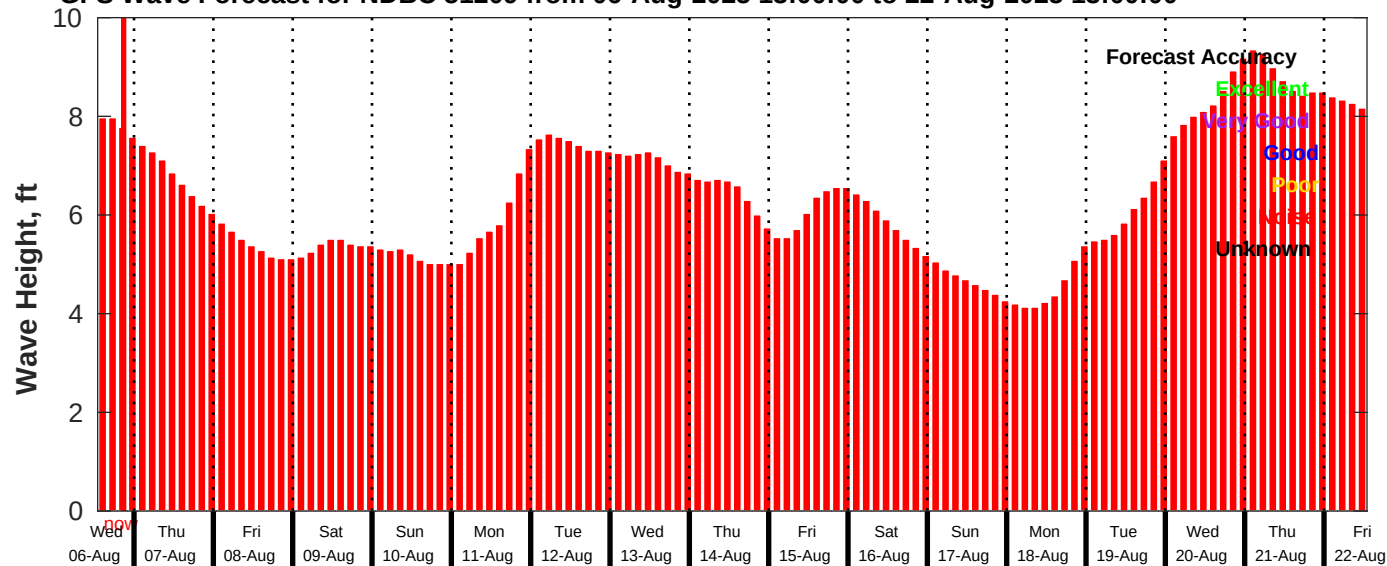
GFS Wave Forecast for NDBC 51209 from 06-Aug-2025 13:00:00 to 22-Aug-2025 13:00:00
