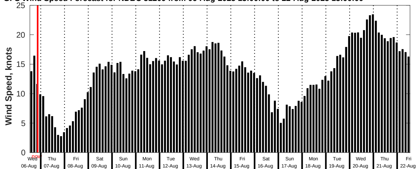
GFS Wind Speed Forecast for NDBC 51209 from 06-Aug-2025 13:00:00 to 22-Aug-2025 13:00:00
