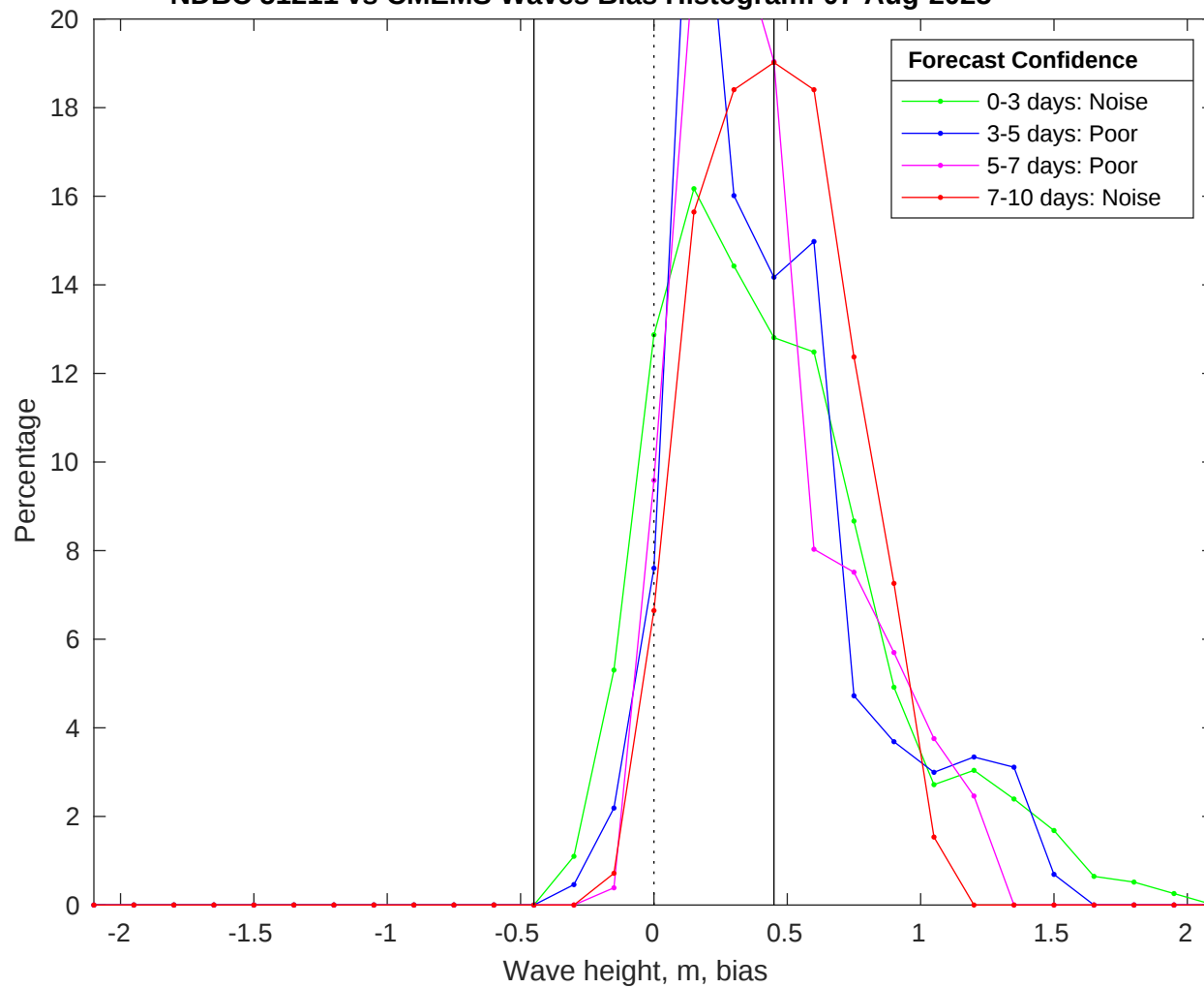
NDBC 51211 vs CMEMS Waves Bias Histogram: 07-Aug-2025
