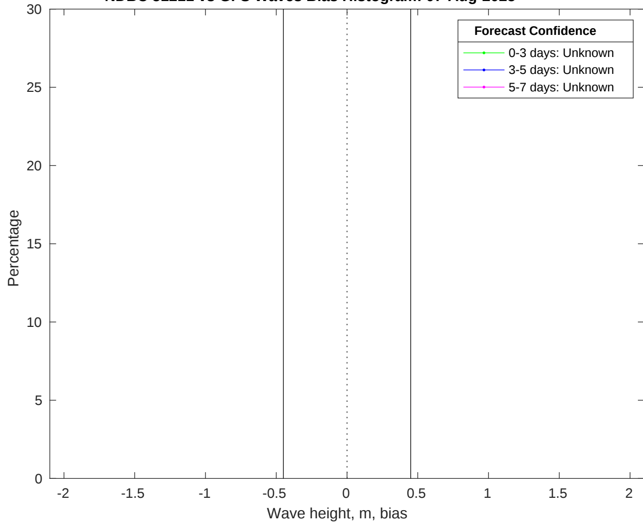
NDBC 51211 vs GFS Waves Bias Histogram: 07-Aug-2025
