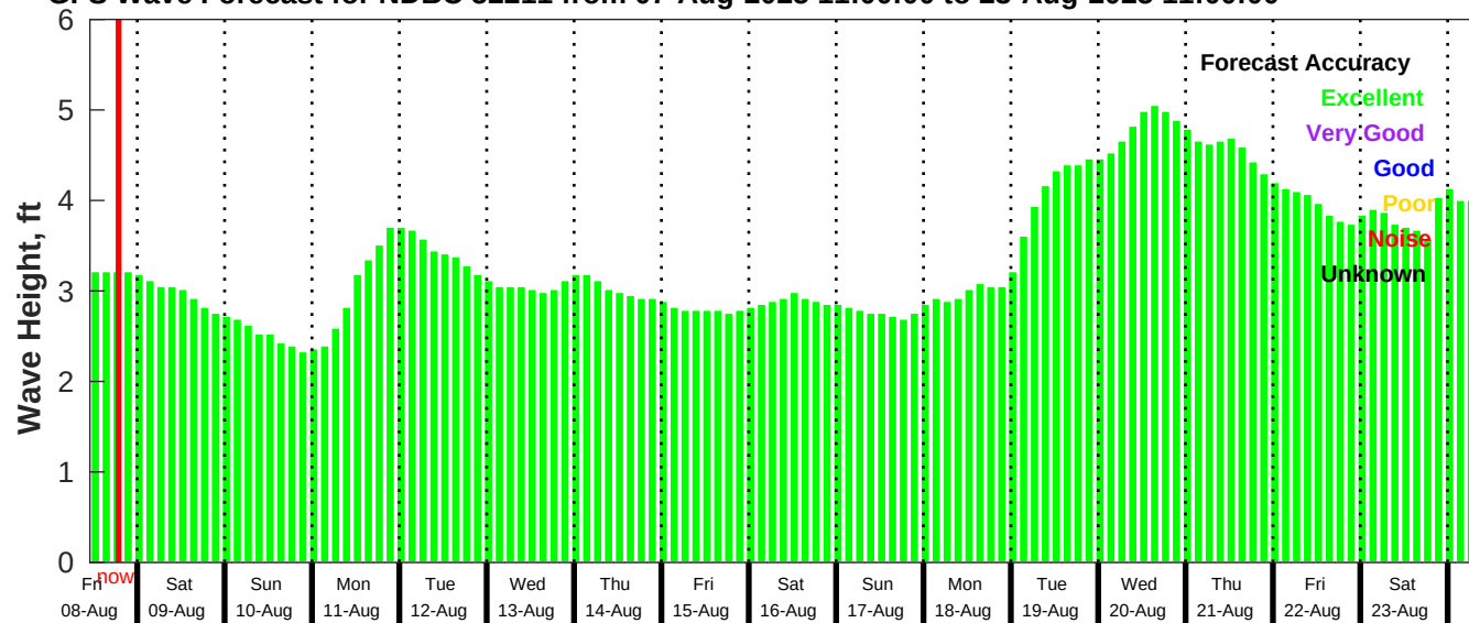
GFS Wave Forecast for NDBC 52211 from 07-Aug-2025 11:00:00 to 23-Aug-2025 11:00:00
