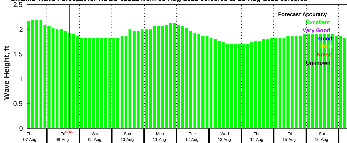
CMEMS Wave Forecast for NDBC 52212 from 06-Aug-2025 09:00:00 to 16-Aug-2025 09:00:00
