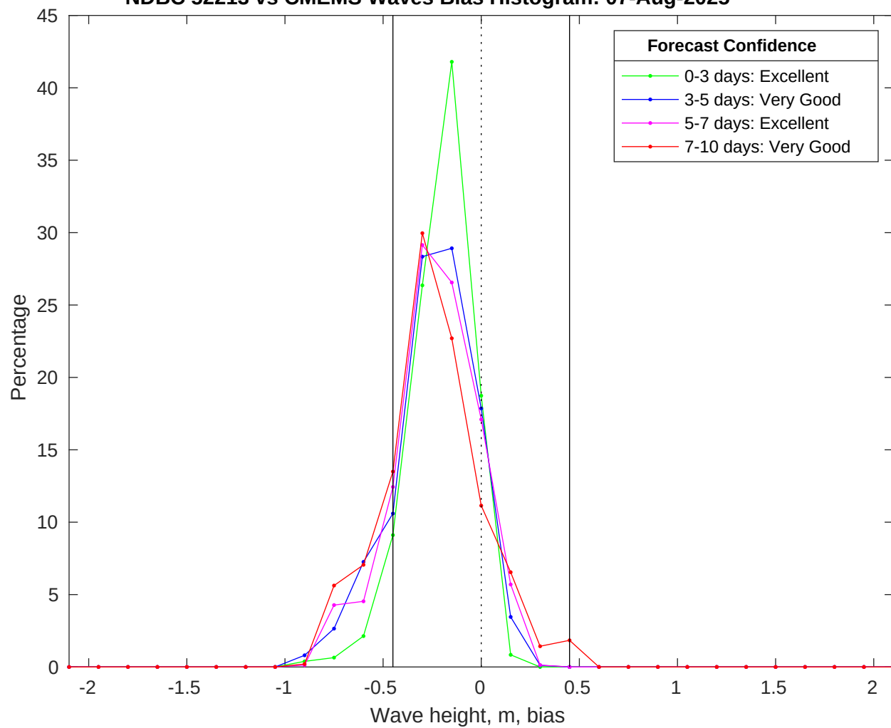
NDBC 52213 vs CMEMS Waves Bias Histogram: 07-Aug-2025
