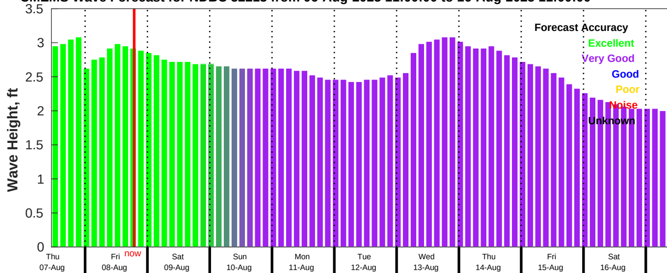
CMEMS Wave Forecast for NDBC 52213 from 06-Aug-2025 11:00:00 to 16-Aug-2025 11:00:00
