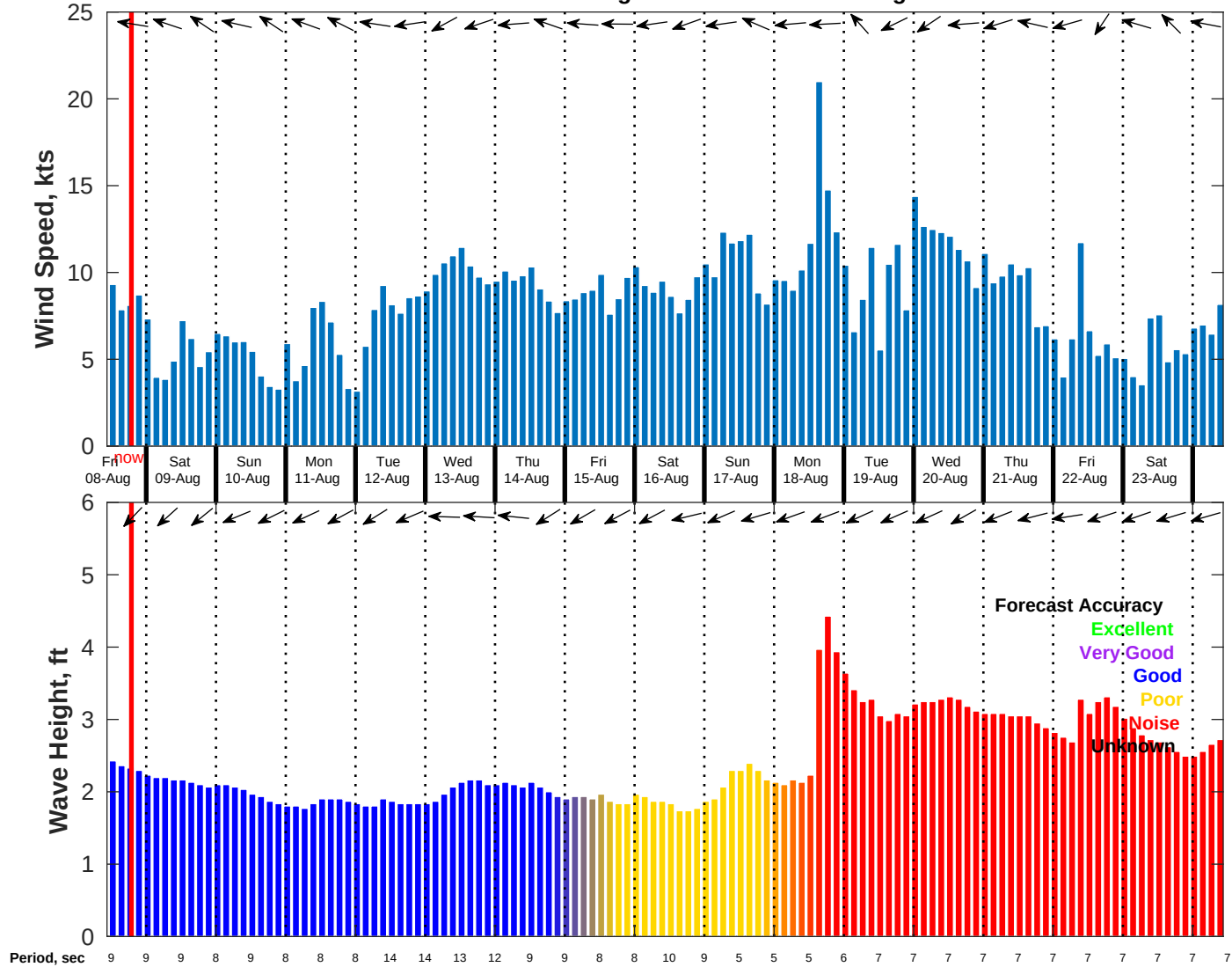
Wind & Wave Forecast for NDBC 52213 from 07-Aug-2025 11:00:00 to 23-Aug-2025 11:00:00
