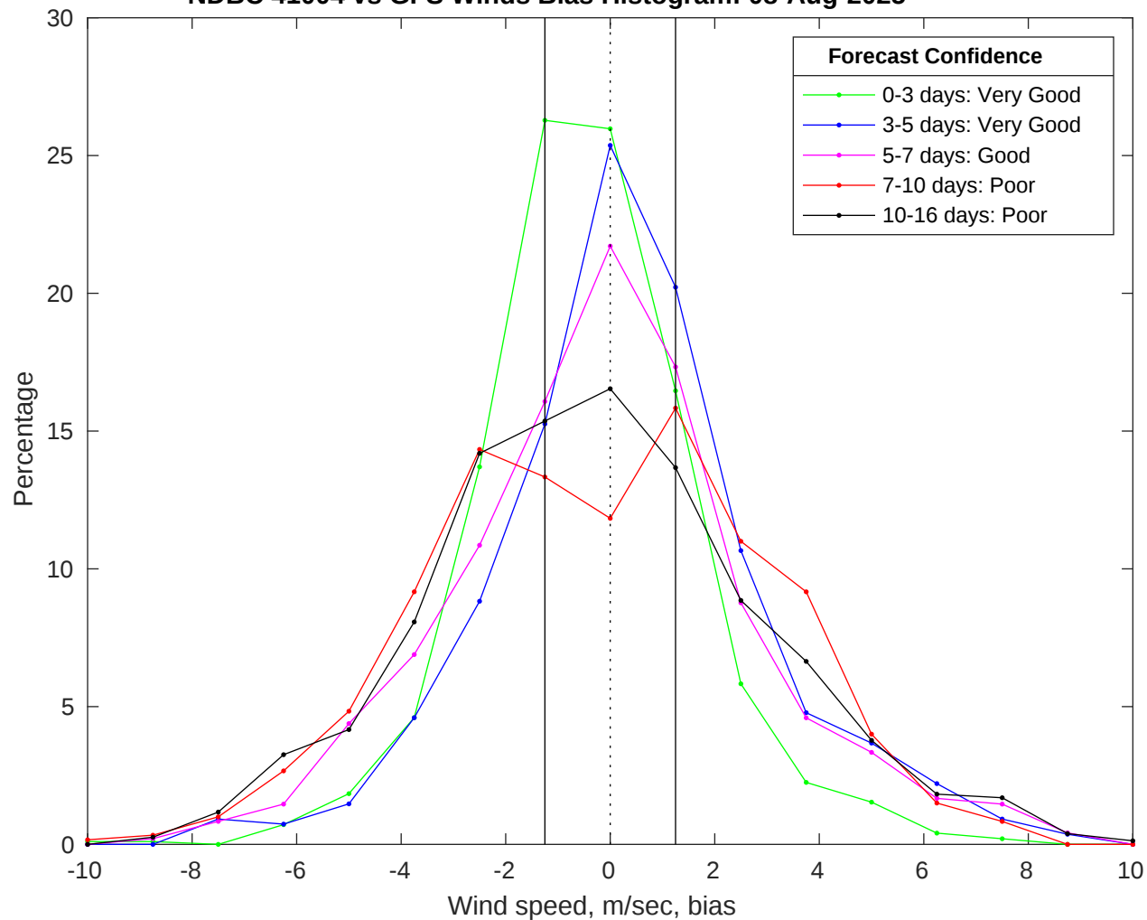
NDBC 41004 vs GFS Winds Bias Histogram: 08-Aug-2025
