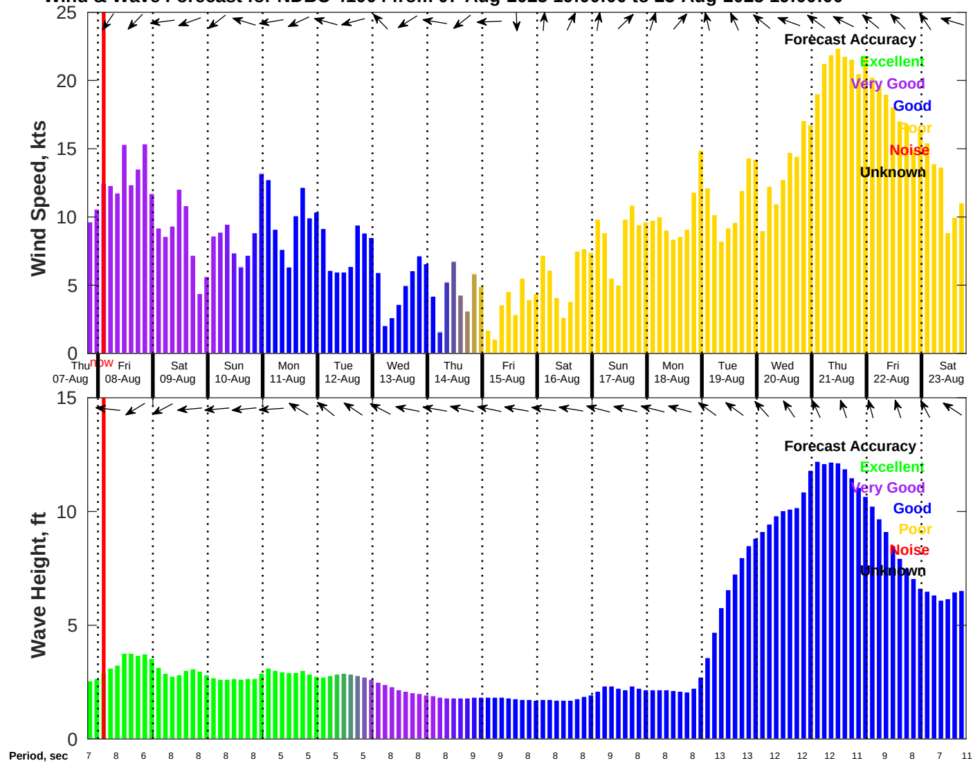
Wind & Wave Forecast for NDBC 41004 from 07-Aug-2025 19:00:00 to 23-Aug-2025 19:00:00
