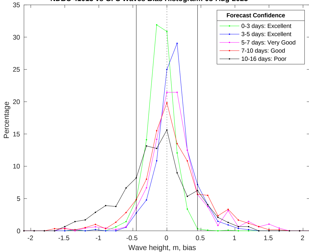
NDBC 41013 vs GFS Waves Bias Histogram: 08-Aug-2025
