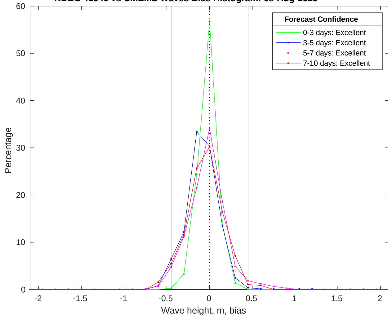
NDBC 41040 vs CMEMS Waves Bias Histogram: 08-Aug-2025
