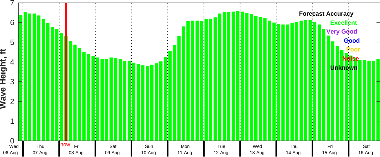
CMEMS Wave Forecast for NDBC 41040 from 06-Aug-2025 21:00:00 to 16-Aug-2025 21:00:00
