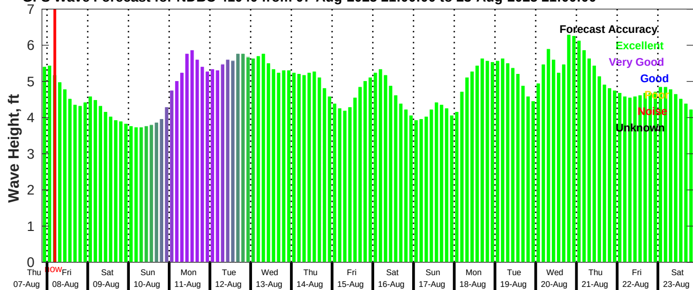
GFS Wave Forecast for NDBC 41040 from 07-Aug-2025 21:00:00 to 23-Aug-2025 21:00:00
