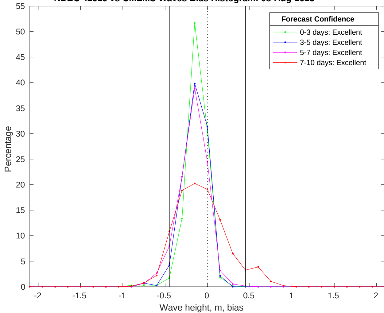
NDBC 42019 vs CMEMS Waves Bias Histogram: 08-Aug-2025
