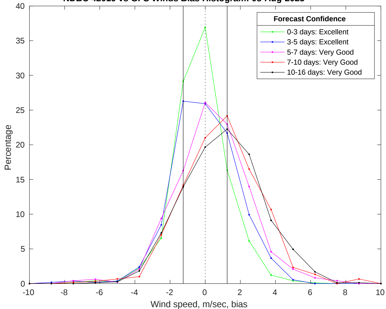
NDBC 42019 vs GFS Winds Bias Histogram: 08-Aug-2025
