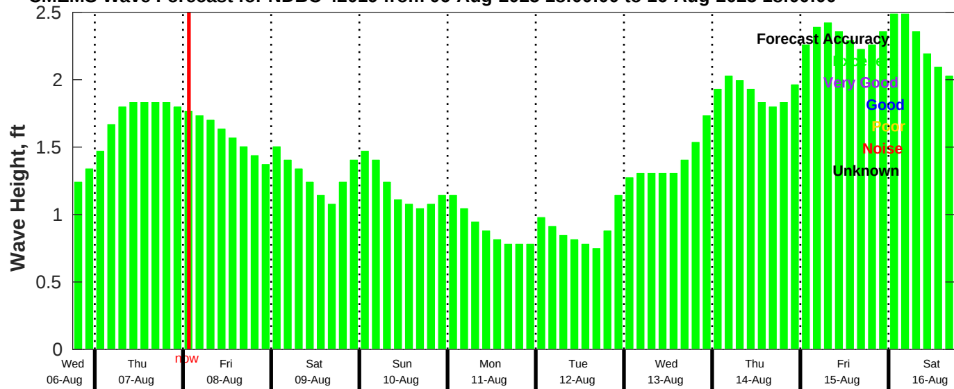
CMEMS Wave Forecast for NDBC 42019 from 06-Aug-2025 18:00:00 to 16-Aug-2025 18:00:00
