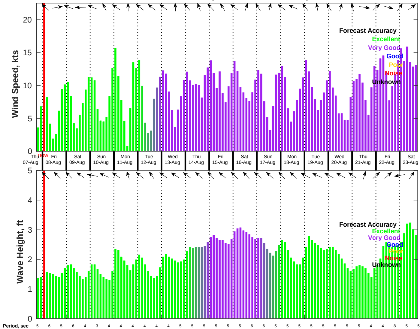
Wind & Wave Forecast for NDBC 42019 from 07-Aug-2025 18:00:00 to 23-Aug-2025 18:00:00
