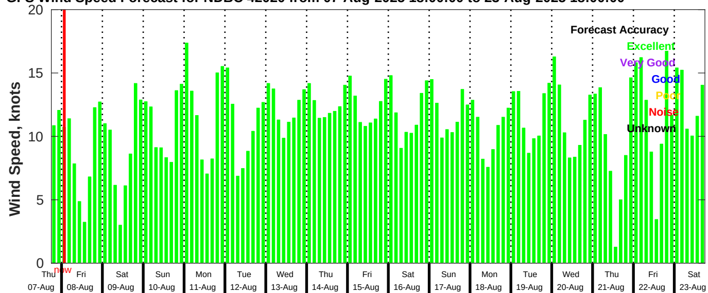
GFS Wind Speed Forecast for NDBC 42020 from 07-Aug-2025 18:00:00 to 23-Aug-2025 18:00:00
