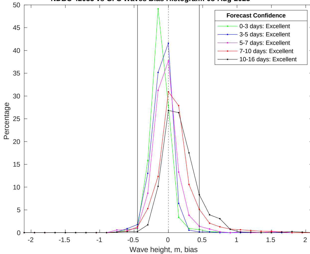
NDBC 42035 vs GFS Waves Bias Histogram: 08-Aug-2025
