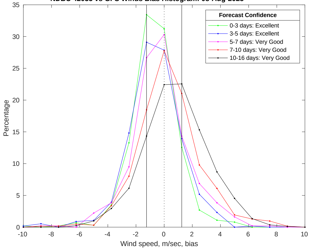
NDBC 42035 vs GFS Winds Bias Histogram: 08-Aug-2025
