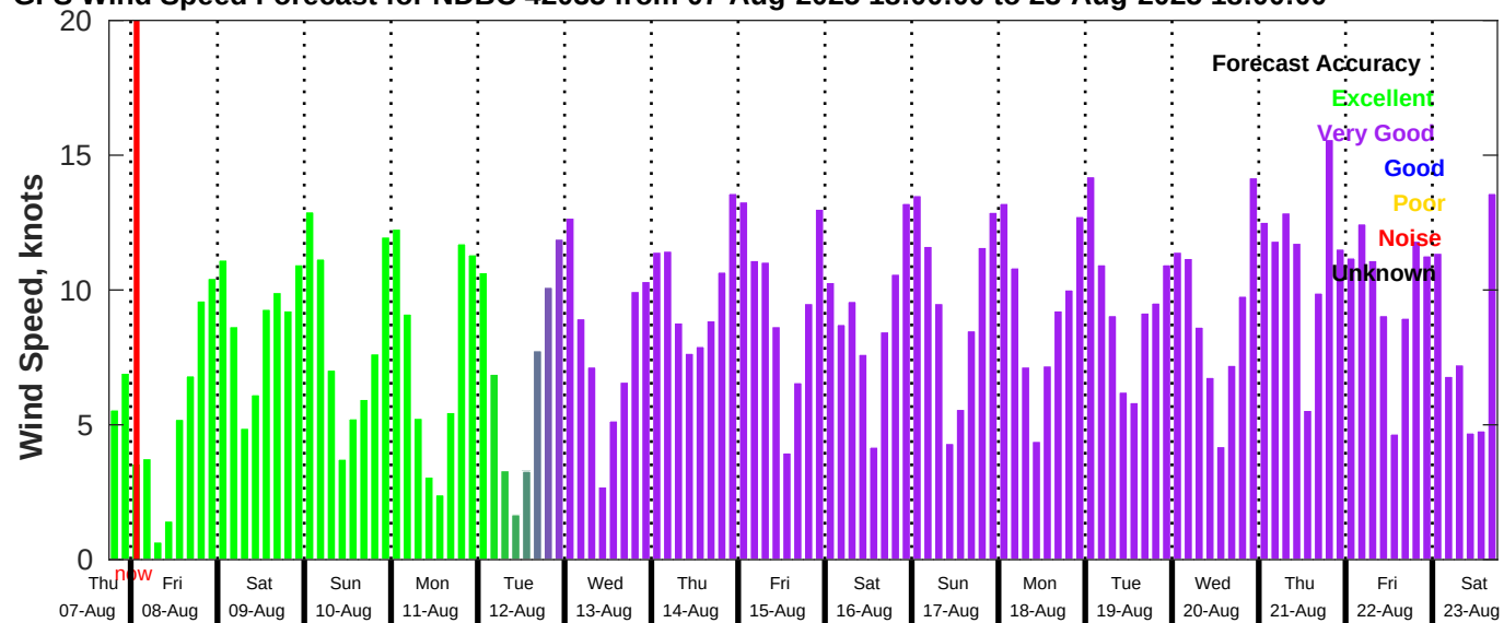
GFS Wind Speed Forecast for NDBC 42035 from 07-Aug-2025 18:00:00 to 23-Aug-2025 18:00:00
