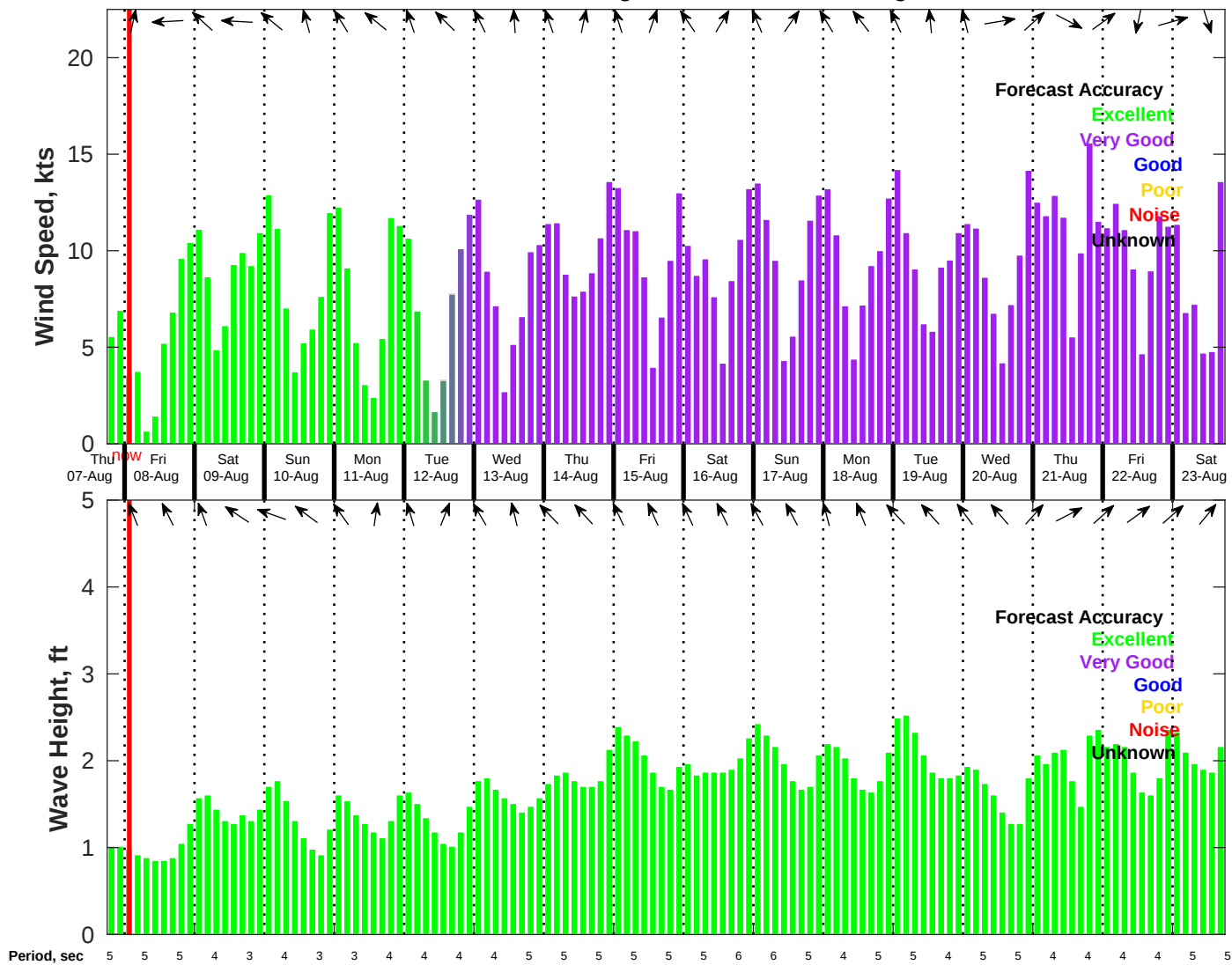
Wind & Wave Forecast for NDBC 42035 from 07-Aug-2025 18:00:00 to 23-Aug-2025 18:00:00
