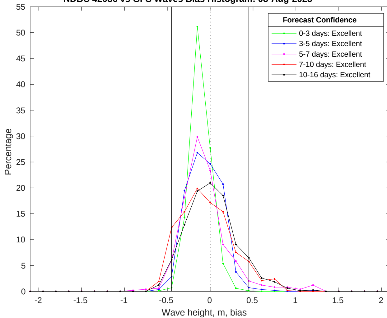
NDBC 42036 vs GFS Waves Bias Histogram: 08-Aug-2025
