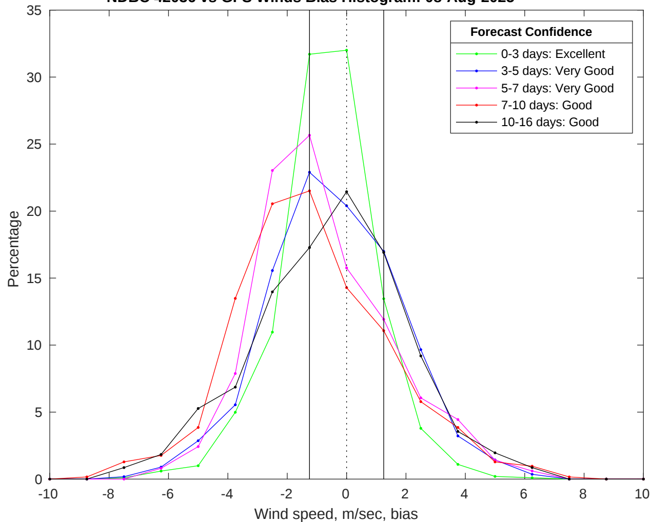
NDBC 42036 vs GFS Winds Bias Histogram: 08-Aug-2025
