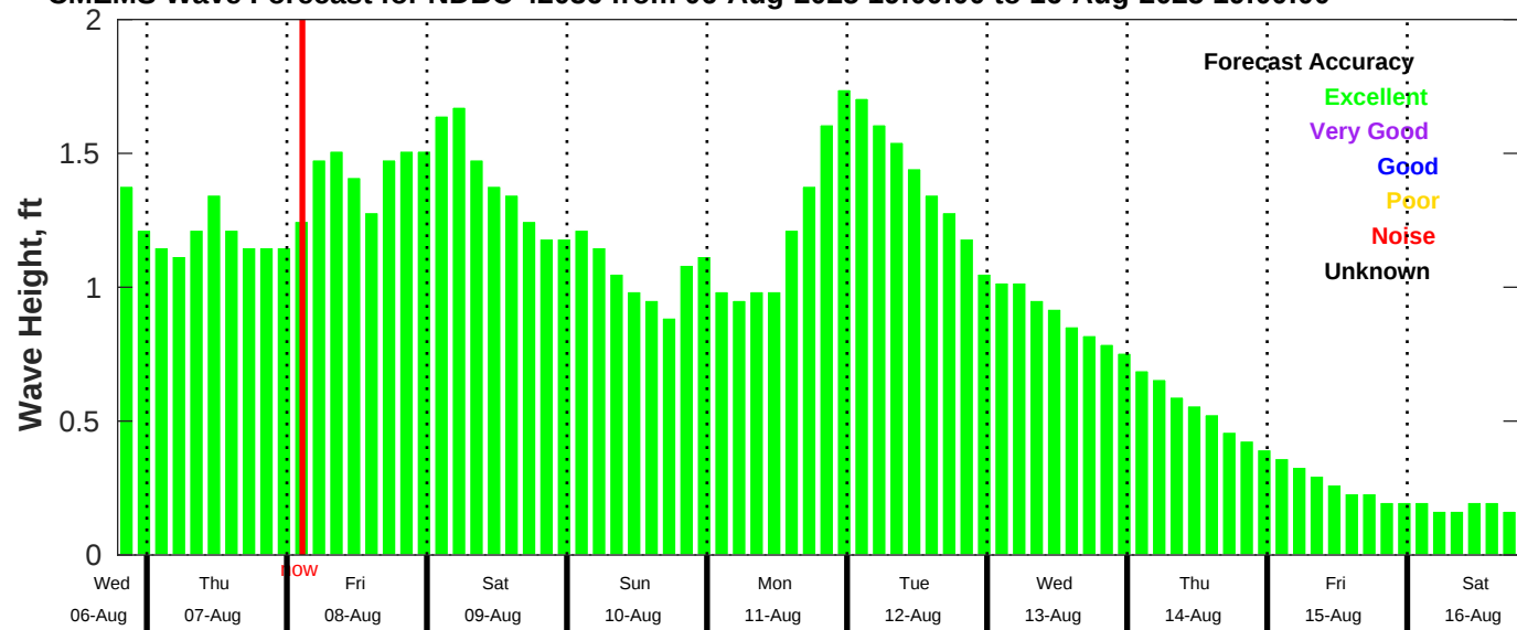
CMEMS Wave Forecast for NDBC 42036 from 06-Aug-2025 19:00:00 to 16-Aug-2025 19:00:00
