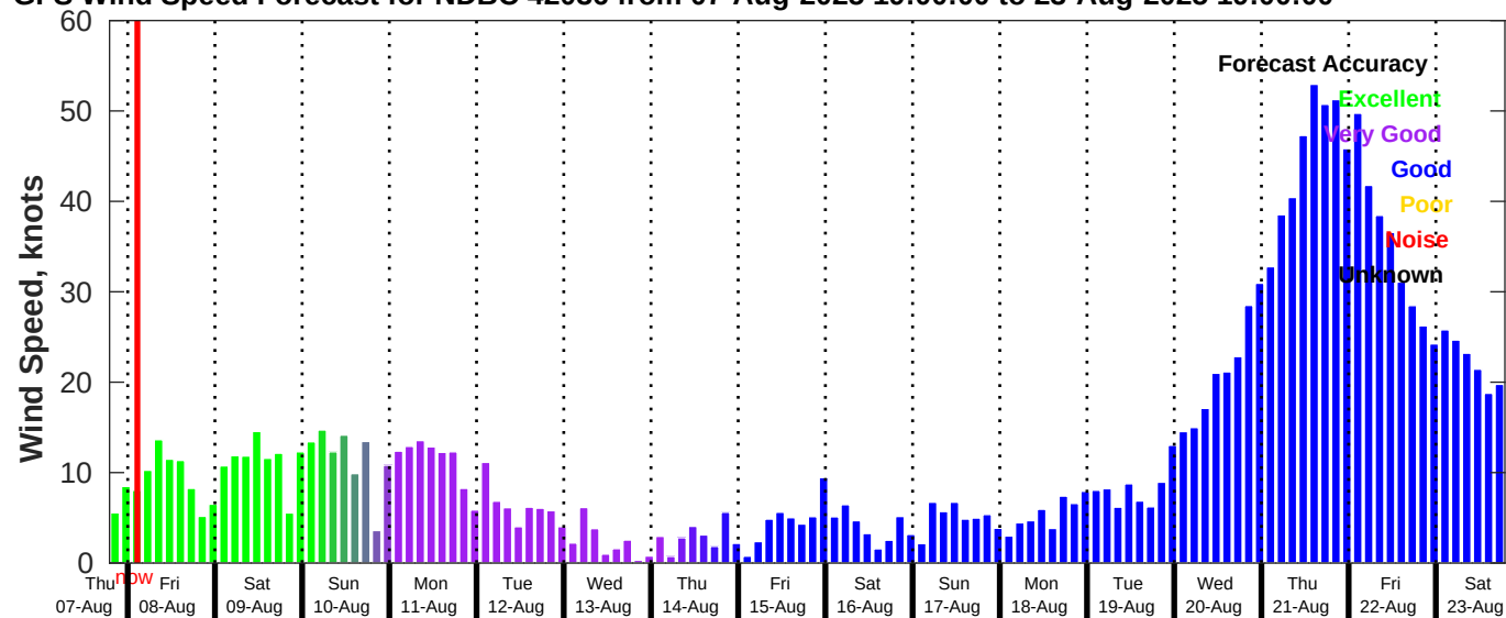
GFS Wind Speed Forecast for NDBC 42036 from 07-Aug-2025 19:00:00 to 23-Aug-2025 19:00:00
