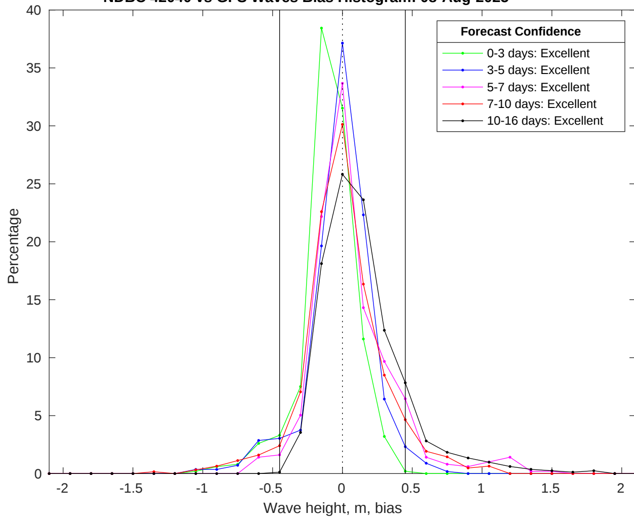
NDBC 42040 vs GFS Waves Bias Histogram: 08-Aug-2025
