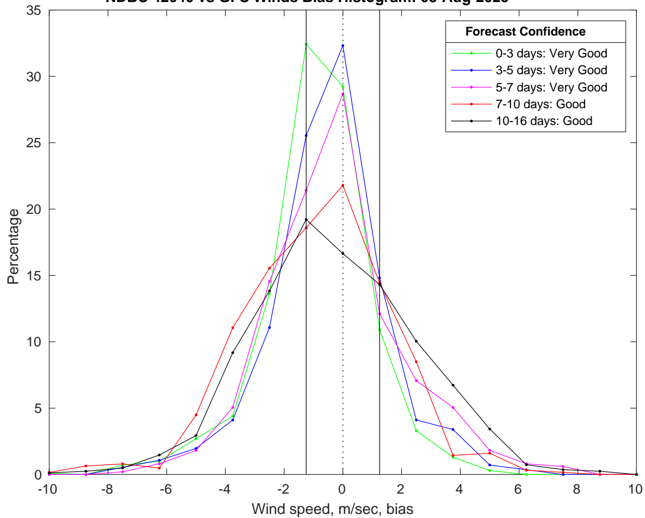
NDBC 42040 vs GFS Winds Bias Histogram: 08-Aug-2025
