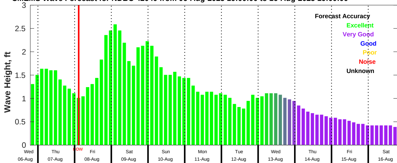
CMEMS Wave Forecast for NDBC 42040 from 06-Aug-2025 19:00:00 to 16-Aug-2025 19:00:00
