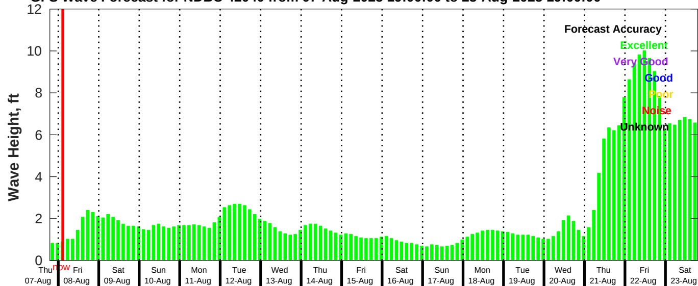
GFS Wave Forecast for NDBC 42040 from 07-Aug-2025 19:00:00 to 23-Aug-2025 19:00:00
