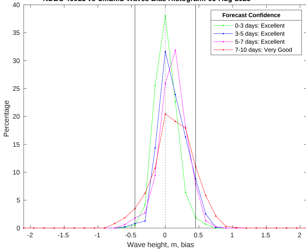
NDBC 46011 vs CMEMS Waves Bias Histogram: 08-Aug-2025
