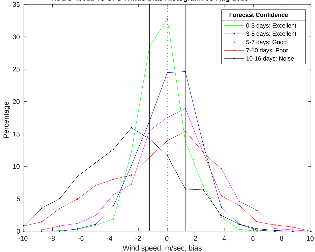
NDBC 46011 vs GFS Winds Bias Histogram: 08-Aug-2025
