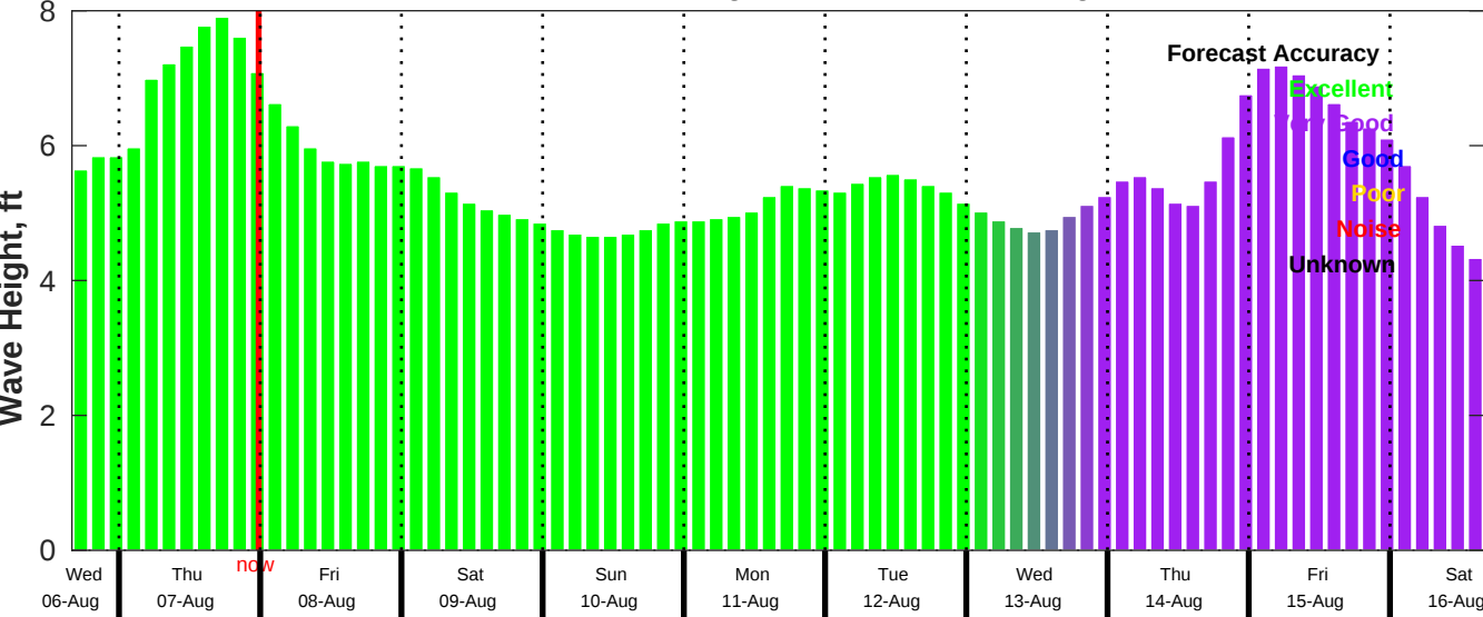
CMEMS Wave Forecast for NDBC 46011 from 06-Aug-2025 16:00:00 to 16-Aug-2025 16:00:00
