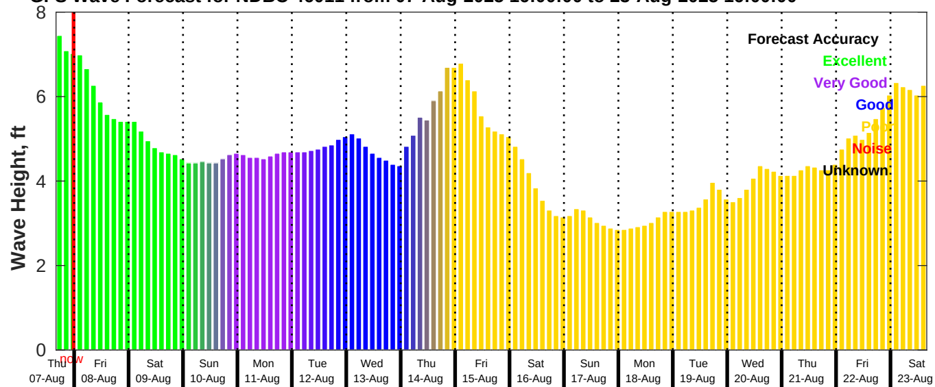
GFS Wave Forecast for NDBC 46011 from 07-Aug-2025 16:00:00 to 23-Aug-2025 16:00:00
