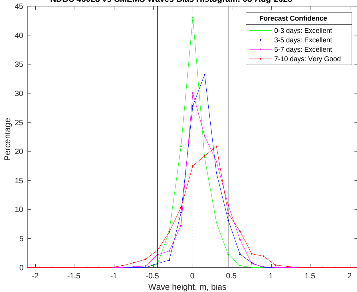
NDBC 46028 vs CMEMS Waves Bias Histogram: 08-Aug-2025
