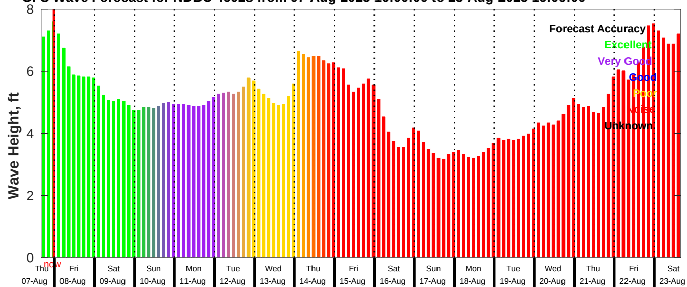
GFS Wave Forecast for NDBC 46028 from 07-Aug-2025 16:00:00 to 23-Aug-2025 16:00:00
